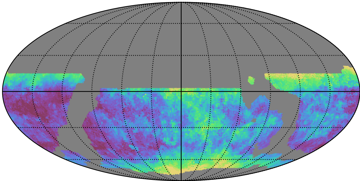
weather_cloudso8v3.4_10yrs WFD g band: Median seeingEff
