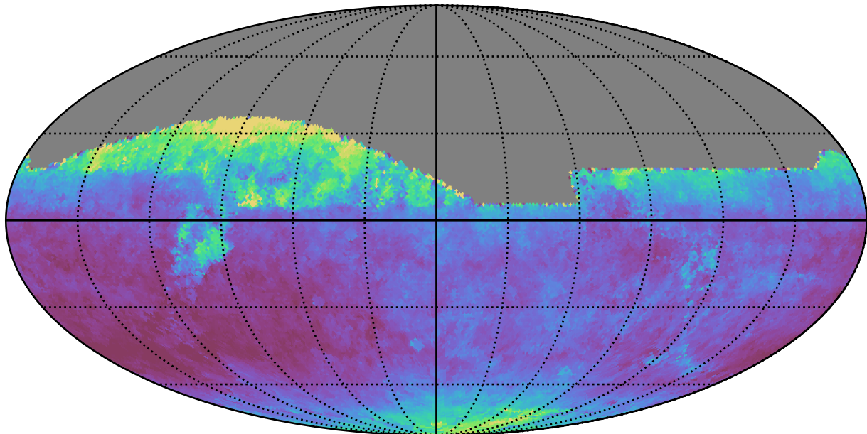
weather_cloudso8v3.4_10yrs All sky z band: Median seeingEff
