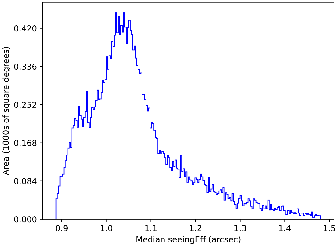
weather_cloudso8v3.4_10yrs All sky z band: Median seeingEff
