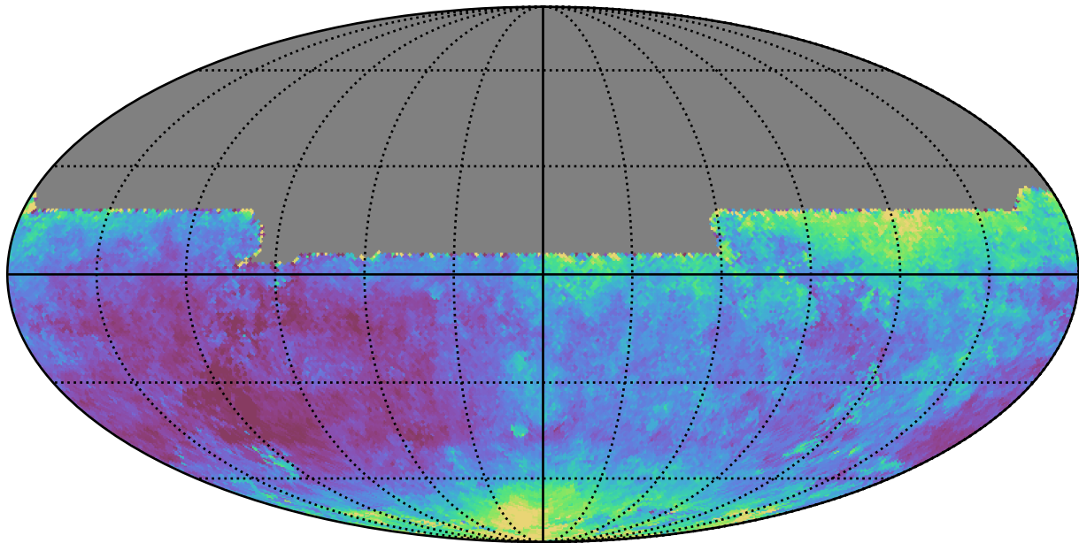
weather_cloudso8v3.4_10yrs All sky y band: Median seeingEff
