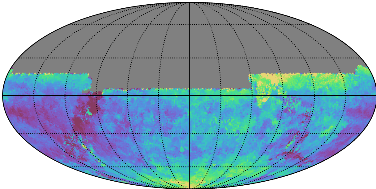
weather_cloudso8v3.4_10yrs All sky u band: Median seeingEff
