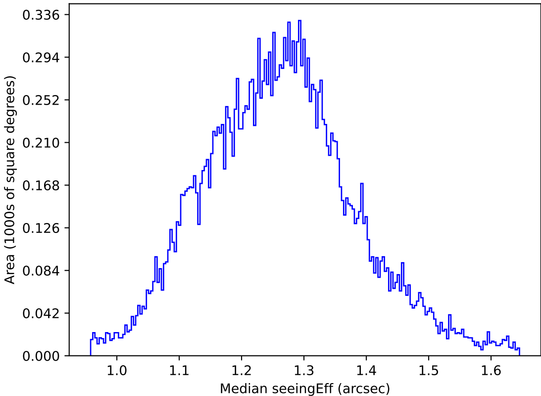
weather_cloudso8v3.4_10yrs All sky u band: Median seeingEff
