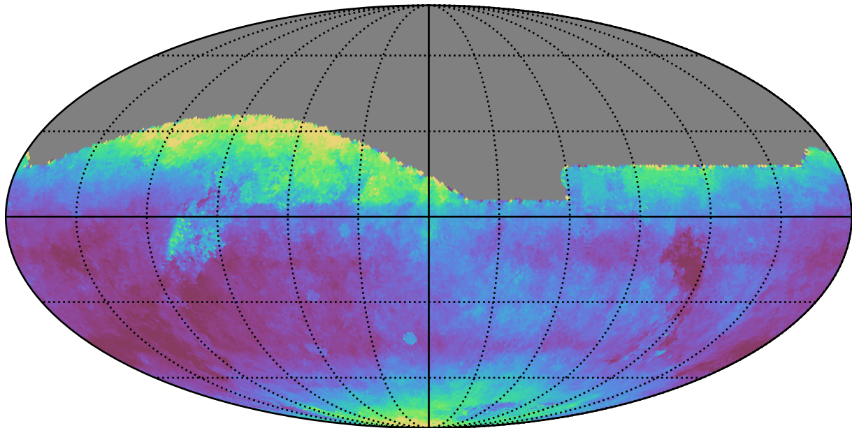
weather_cloudso8v3.4_10yrs All sky r band: Median seeingEff
