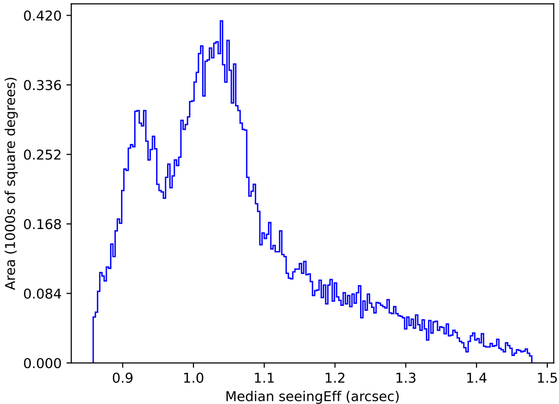
weather_cloudso8v3.4_10yrs All sky i band: Median seeingEff
