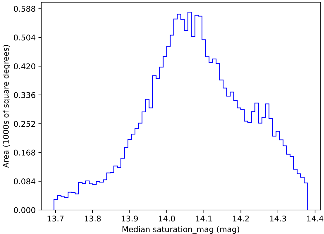
weather_cloudso8v3.4_10yrs WFD z band: Median saturation_mag
