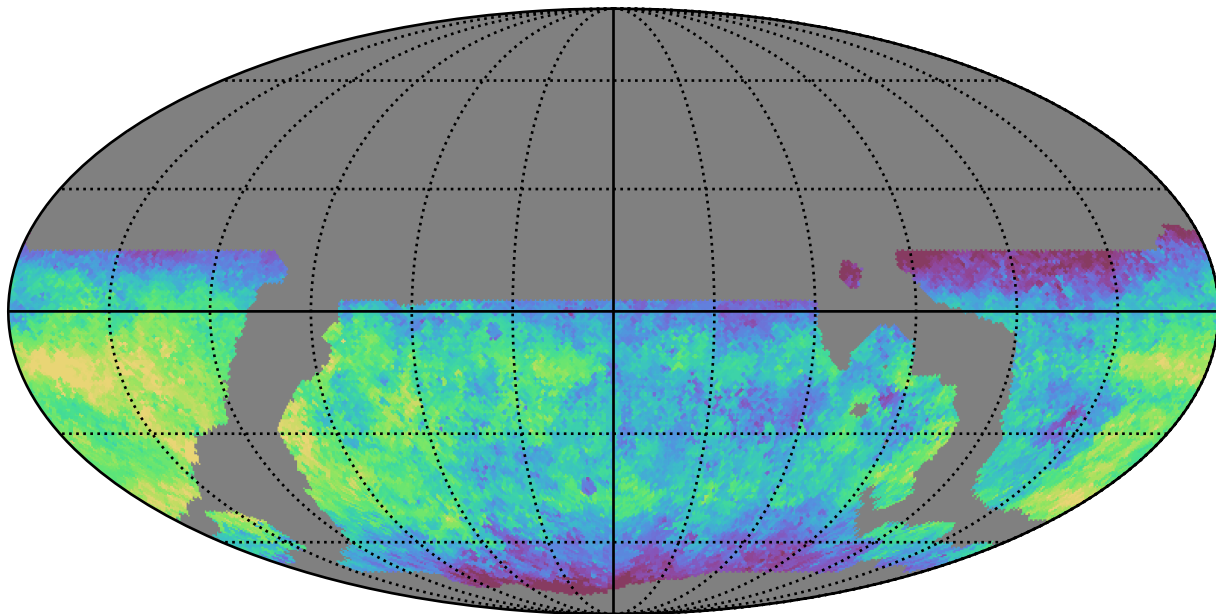
weather_cloudso8v3.4_10yrs WFD u band: Median saturation_mag
