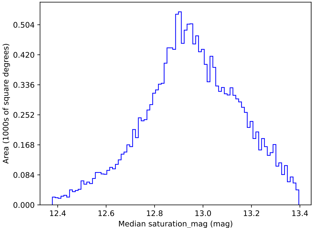
weather_cloudso8v3.4_10yrs WFD u band: Median saturation_mag
