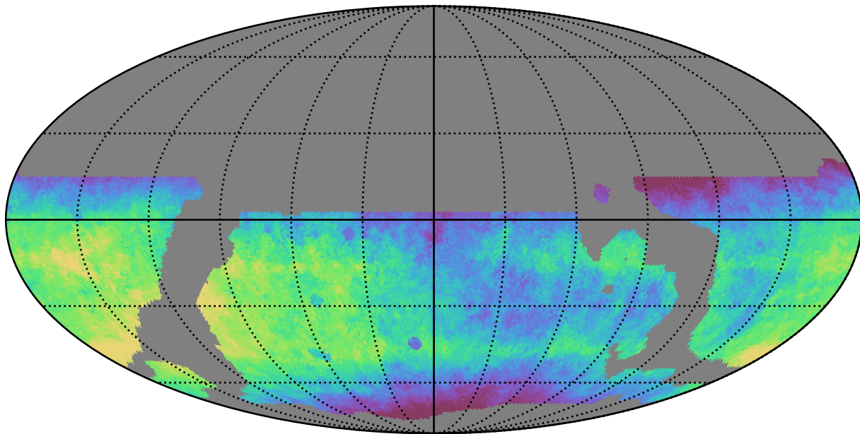
weather_cloudso8v3.4_10yrs WFD r band: Median saturation_mag
