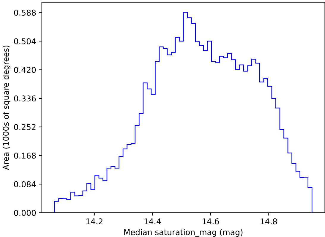
weather_cloudso8v3.4_10yrs WFD r band: Median saturation_mag
