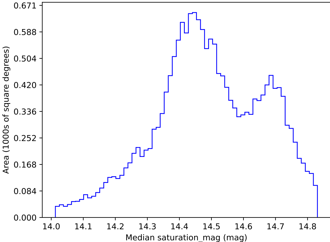
weather_cloudso8v3.4_10yrs WFD i band: Median saturation_mag
