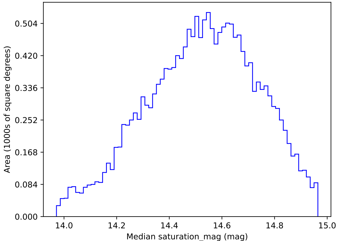
weather_cloudso8v3.4_10yrs WFD g band: Median saturation_mag
