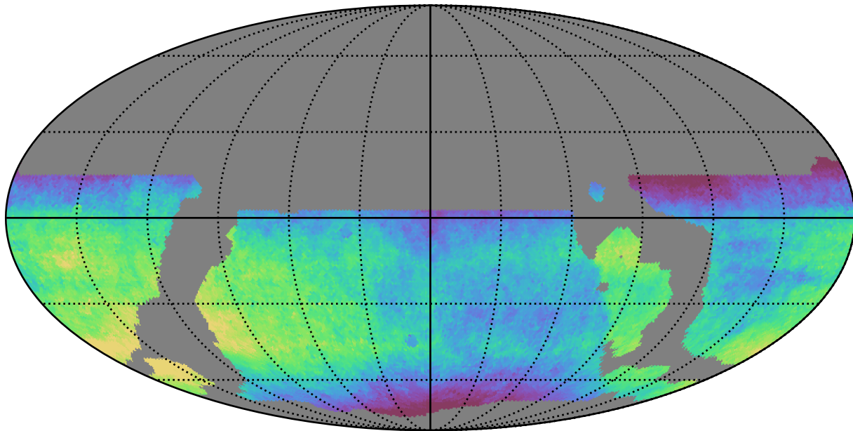
weather_cloudso8v3.4_10yrs WFD all bands: Median saturation_mag
