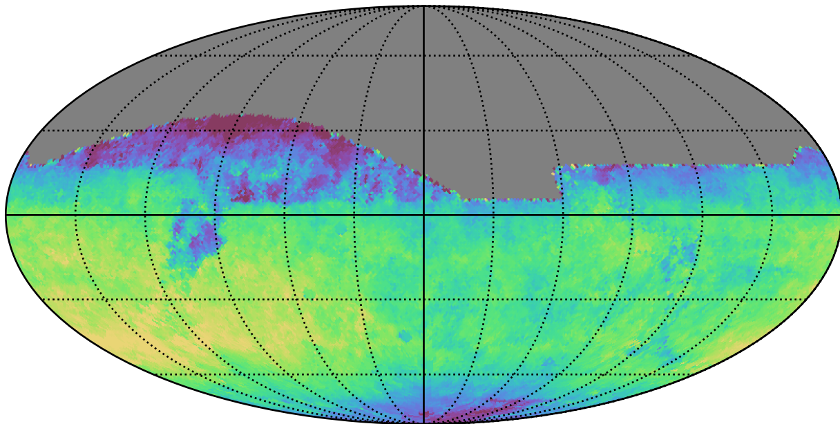
weather_cloudso8v3.4_10yrs All sky z band: Median saturation_mag
