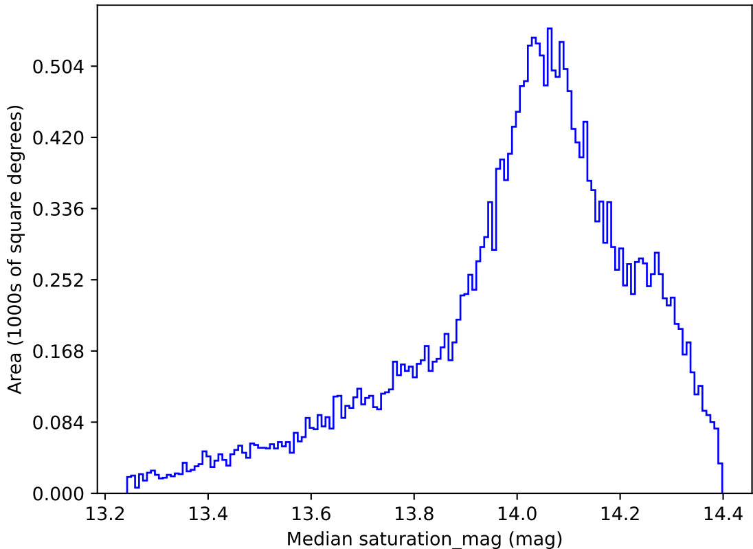
weather_cloudso8v3.4_10yrs All sky z band: Median saturation_mag
