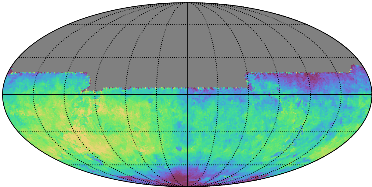
weather_cloudso8v3.4_10yrs All sky y band: Median saturation_mag
