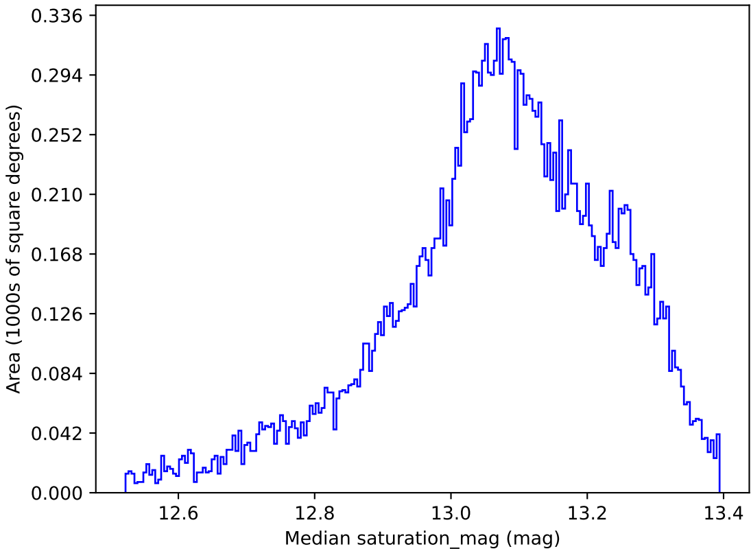
weather_cloudso8v3.4_10yrs All sky y band: Median saturation_mag
