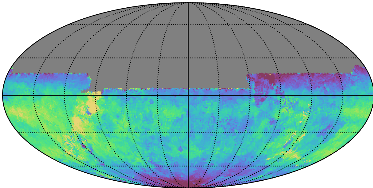
weather_cloudso8v3.4_10yrs All sky u band: Median saturation_mag
