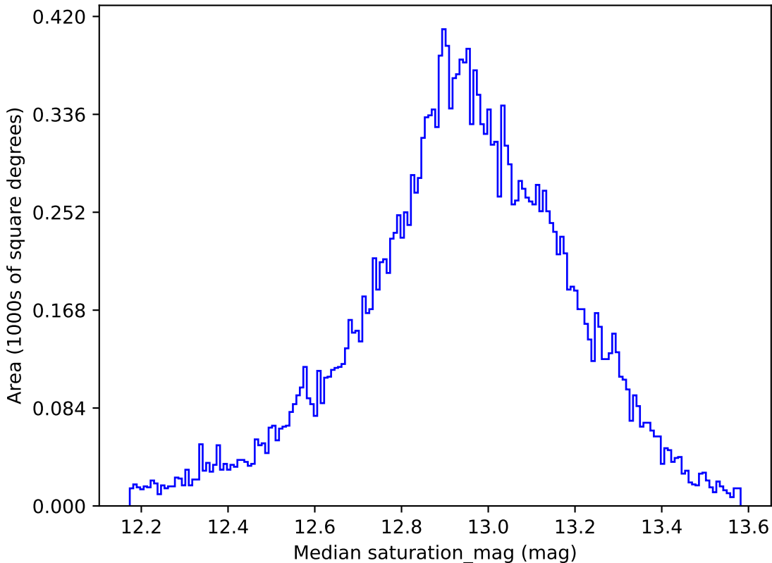
weather_cloudso8v3.4_10yrs All sky u band: Median saturation_mag
