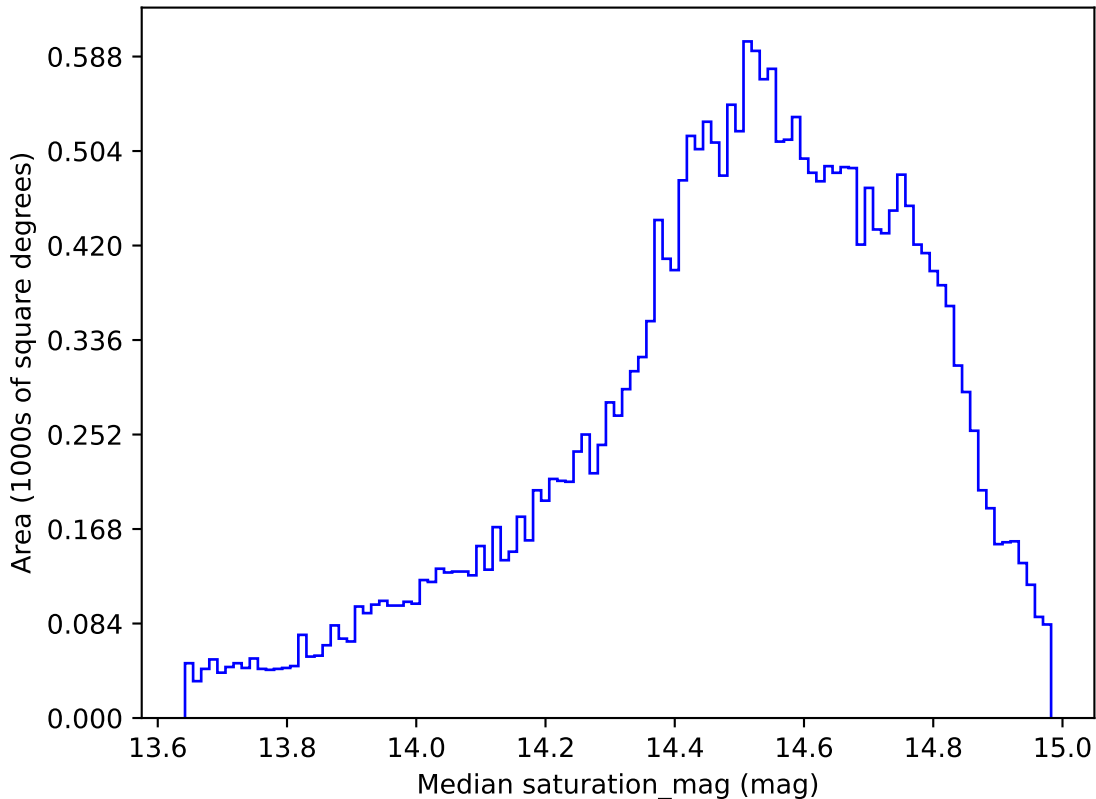
weather_cloudso8v3.4_10yrs All sky r band: Median saturation_mag
