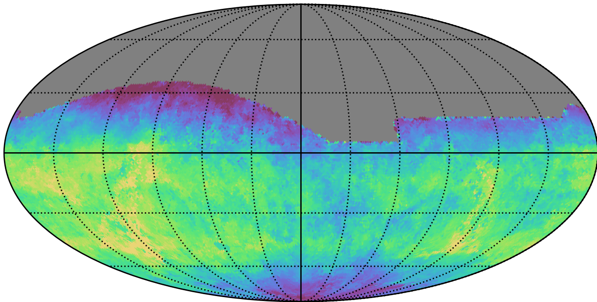
weather_cloudso8v3.4_10yrs All sky g band: Median saturation_mag
