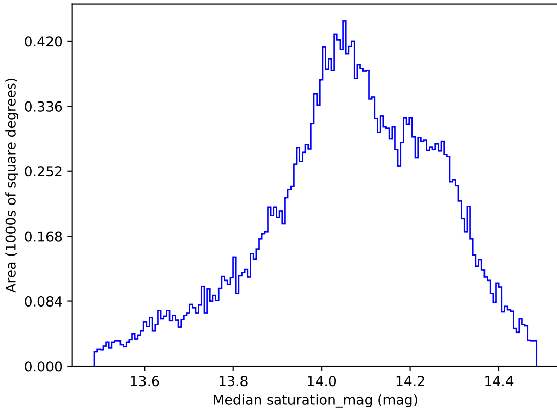
weather_cloudso8v3.4_10yrs All sky all bands: Median saturation_mag
