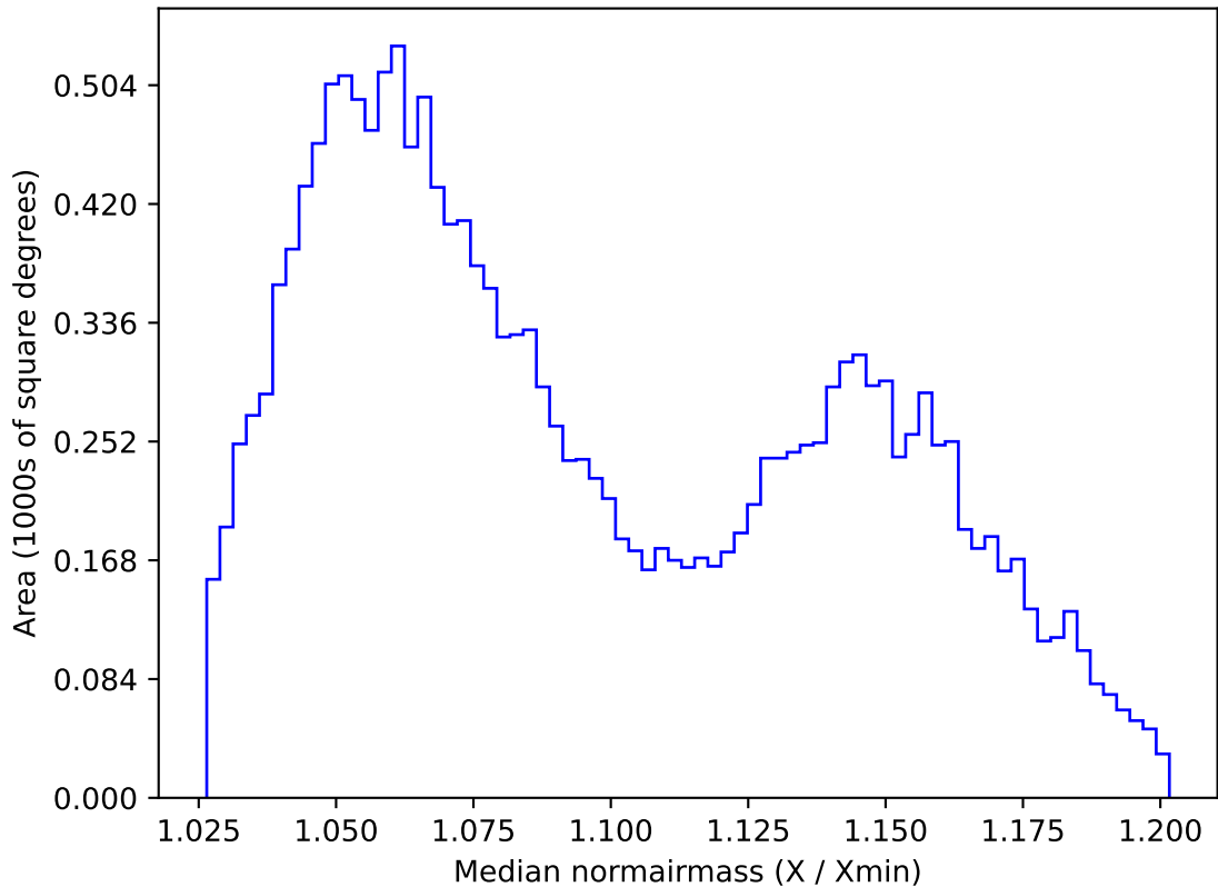
weather_cloudso8v3.4_10yrs WFD z band: Median normairmass
