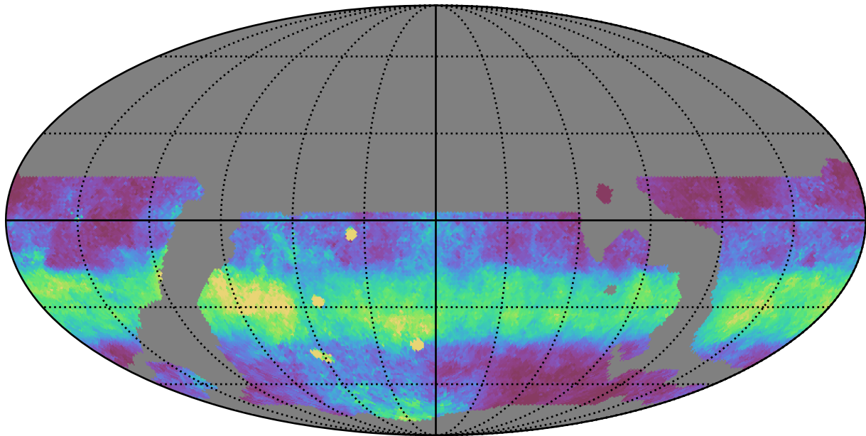
weather_cloudso8v3.4_10yrs WFD y band: Median normairmass
