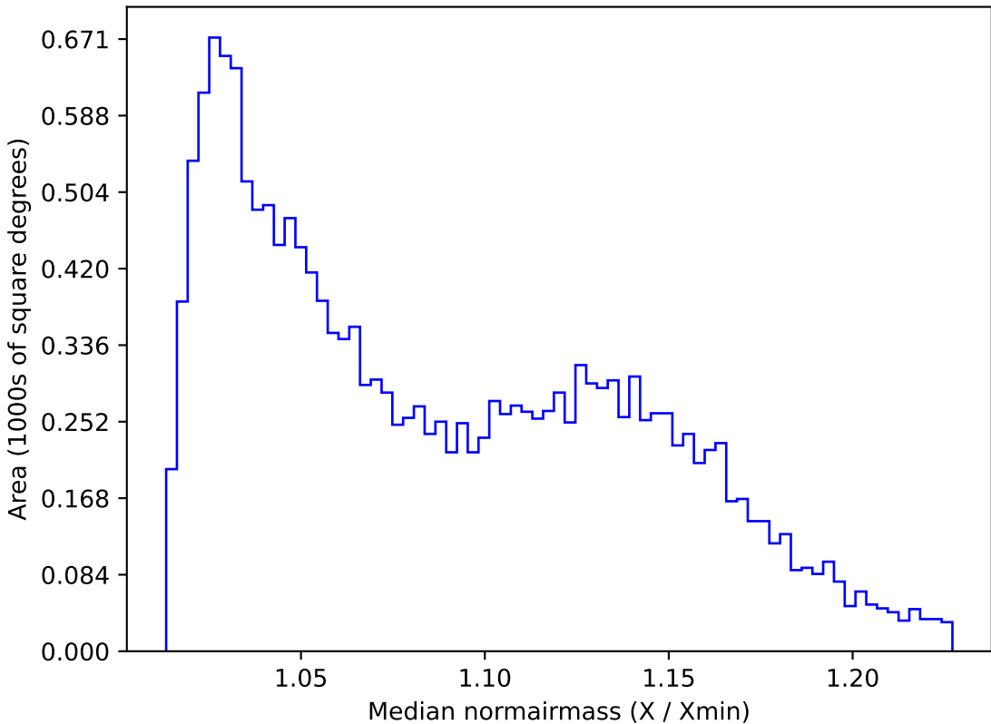
weather_cloudso8v3.4_10yrs WFD u band: Median normairmass
