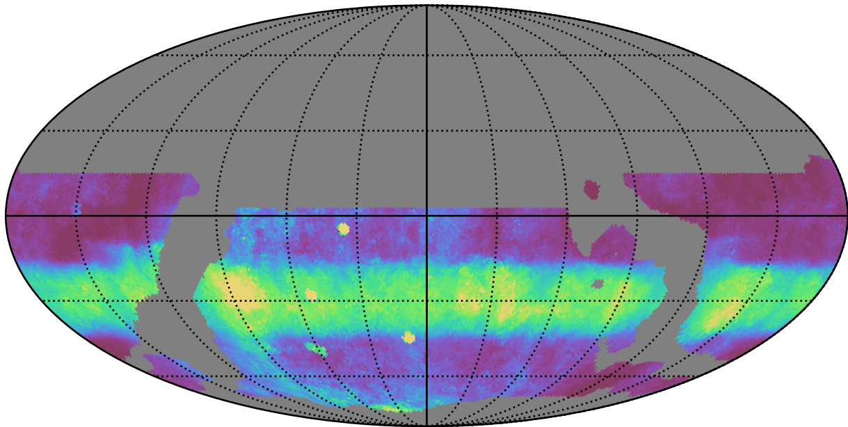
weather_cloudso8v3.4_10yrs WFD r band: Median normairmass
