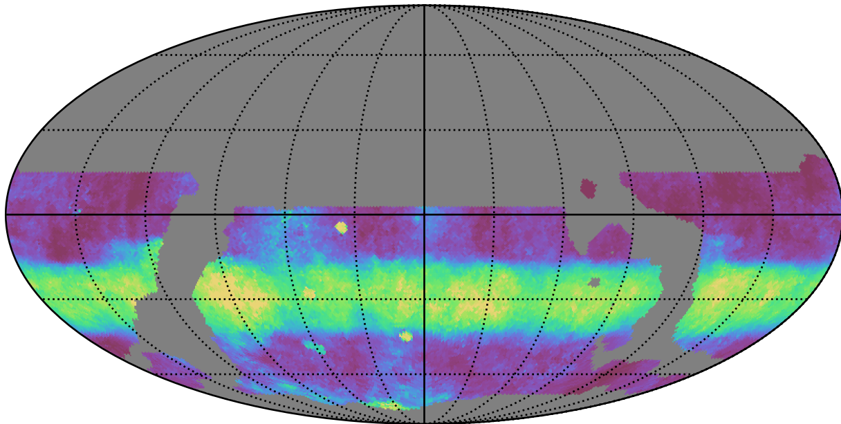
weather_cloudso8v3.4_10yrs WFD i band: Median normairmass
