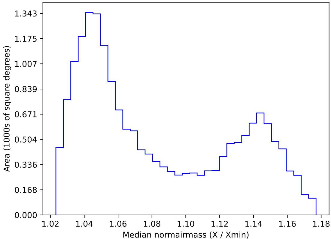
weather_cloudso8v3.4_10yrs WFD i band: Median normairmass
