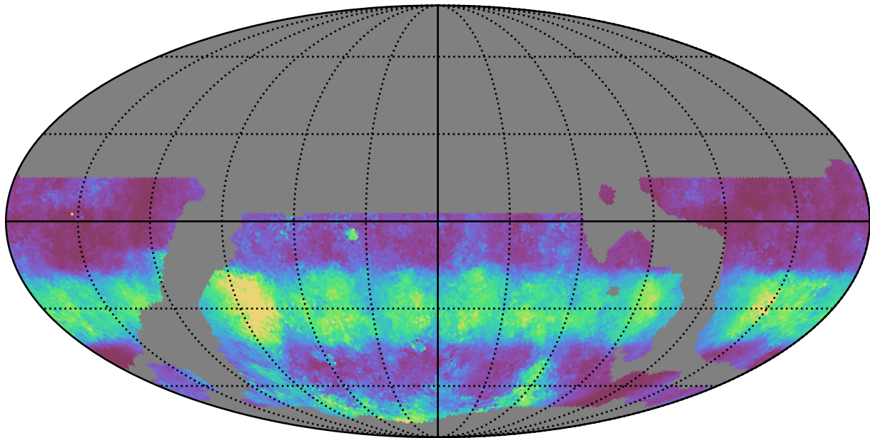
weather_cloudso8v3.4_10yrs WFD g band: Median normairmass
