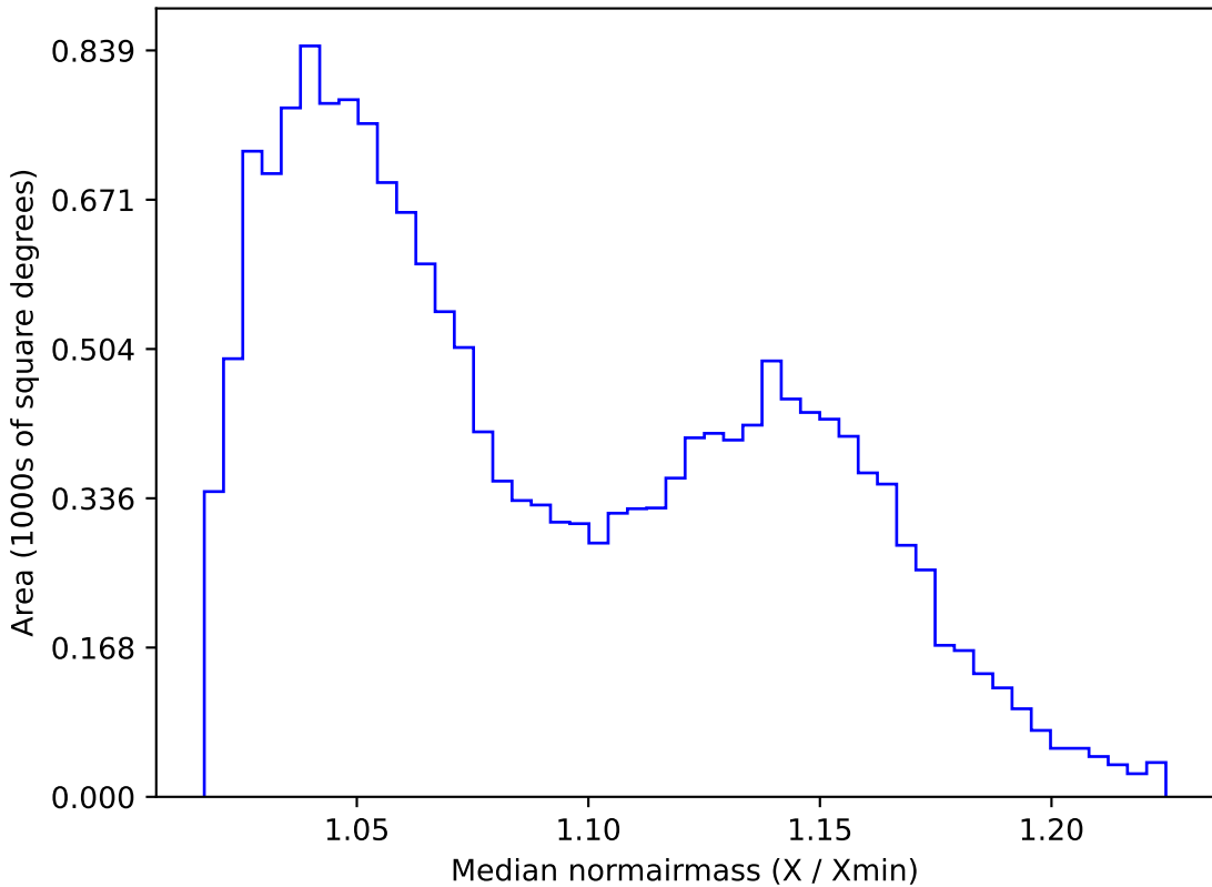
weather_cloudso8v3.4_10yrs WFD g band: Median normairmass
