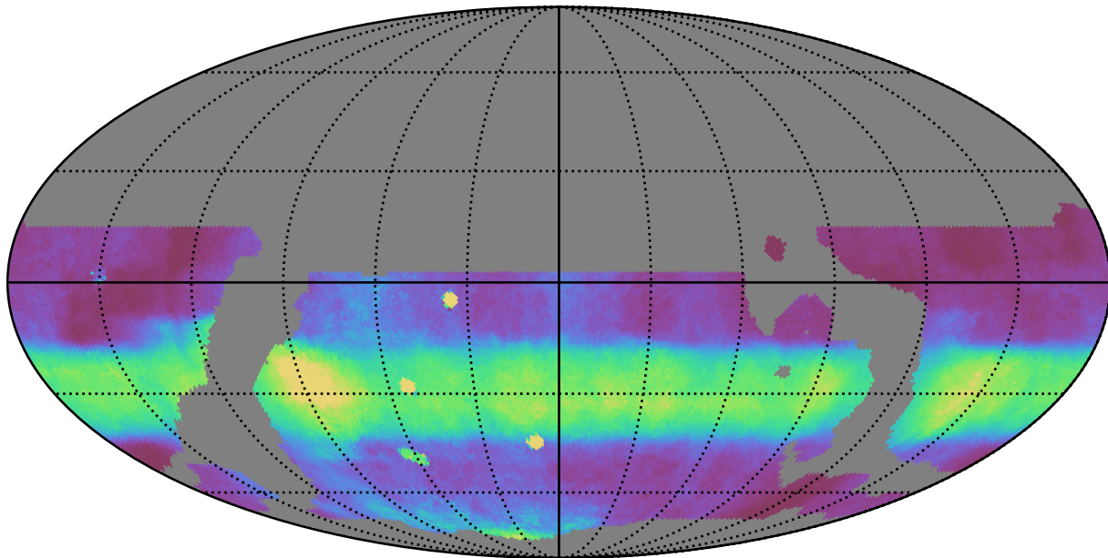
weather_cloudso8v3.4_10yrs WFD all bands: Median normairmass
