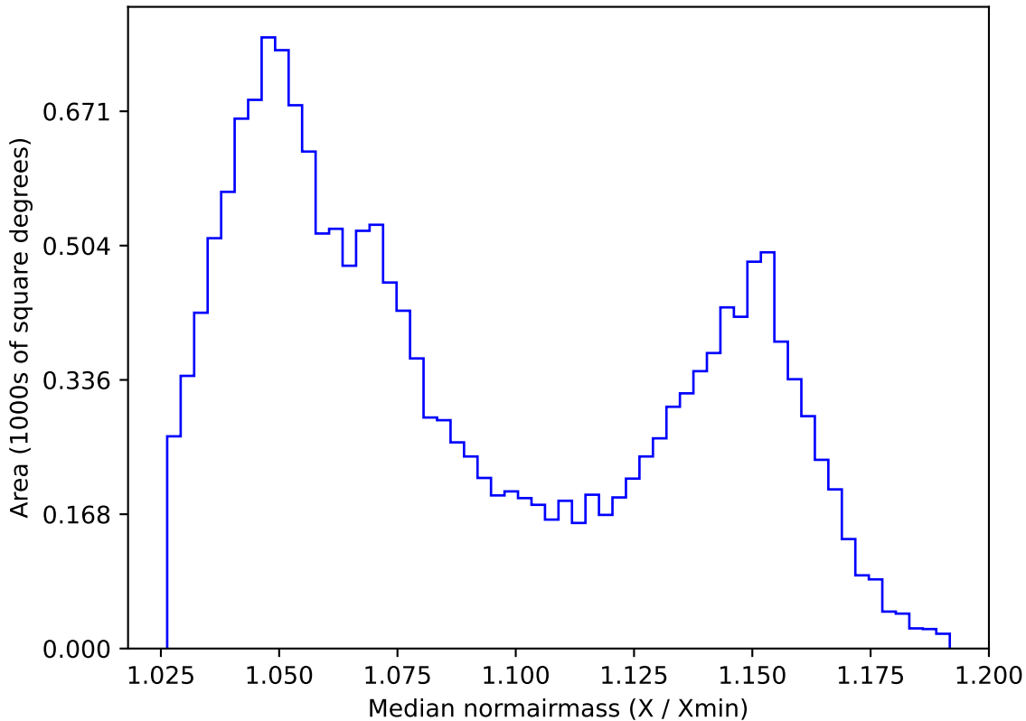
weather_cloudso8v3.4_10yrs WFD all bands: Median normairmass
