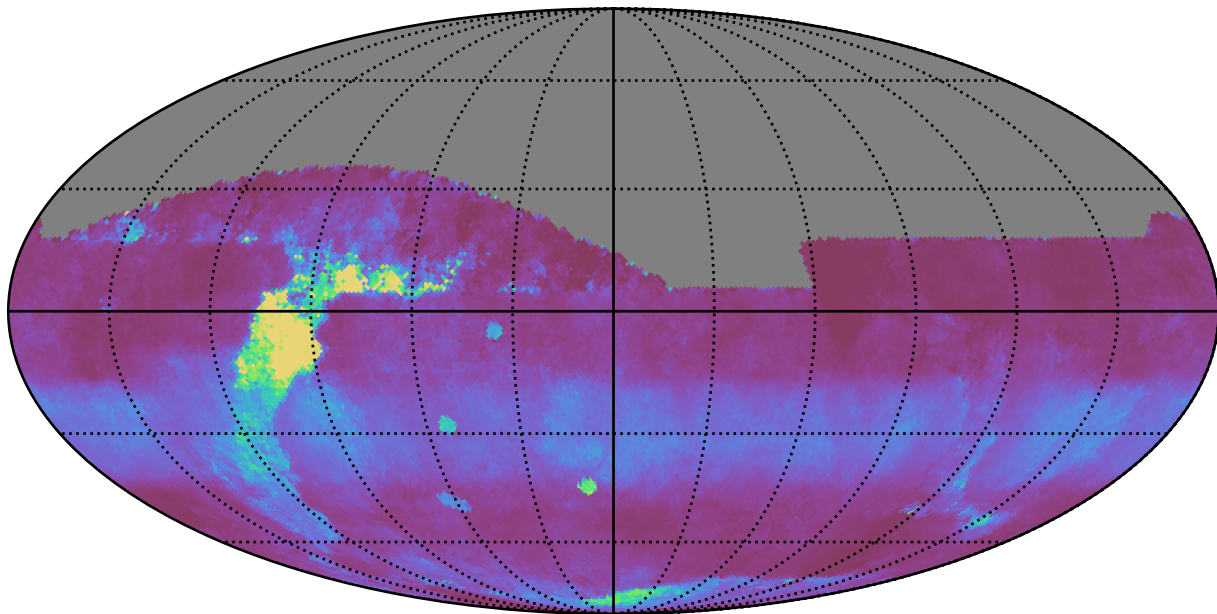
weather_cloudso8v3.4_10yrs All sky z band: Median normairmass
