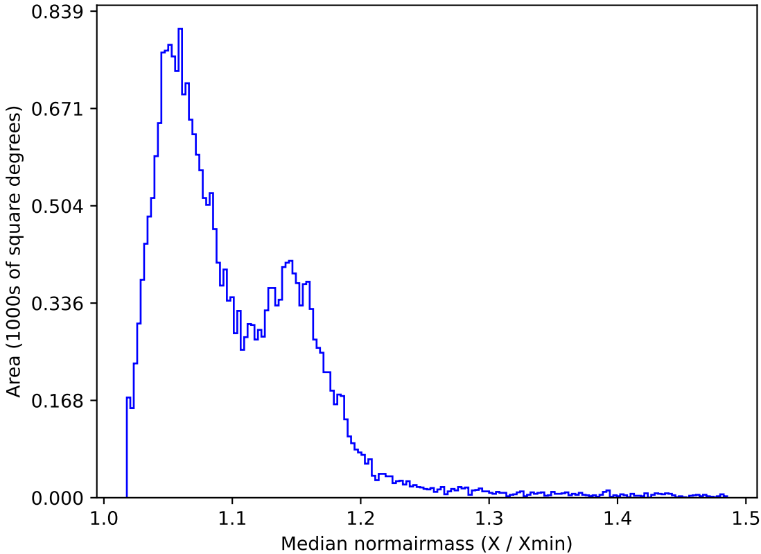
weather_cloudso8v3.4_10yrs All sky z band: Median normairmass
