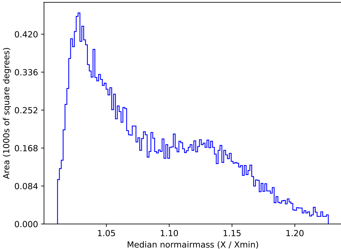
weather_cloudso8v3.4_10yrs All sky u band: Median normairmass
