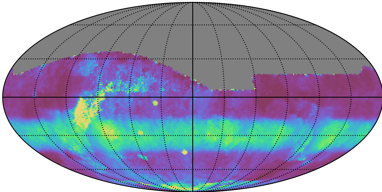
weather_cloudso8v3.4_10yrs All sky r band: Median normairmass
