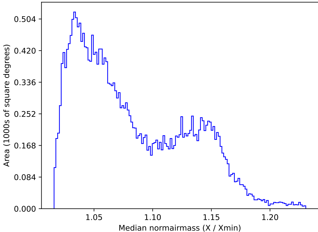
weather_cloudso8v3.4_10yrs All sky r band: Median normairmass
