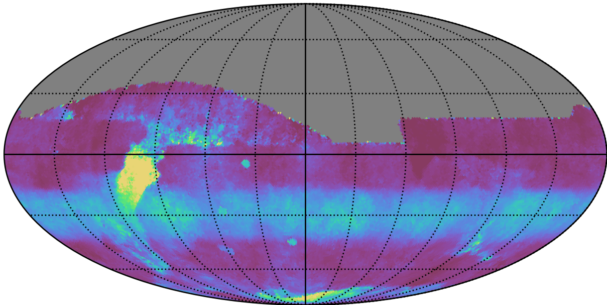
weather_cloudso8v3.4_10yrs All sky i band: Median normairmass
