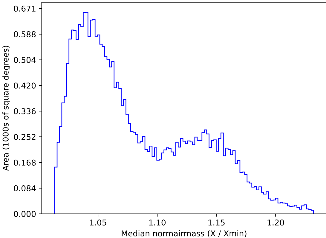
weather_cloudso8v3.4_10yrs All sky g band: Median normairmass
