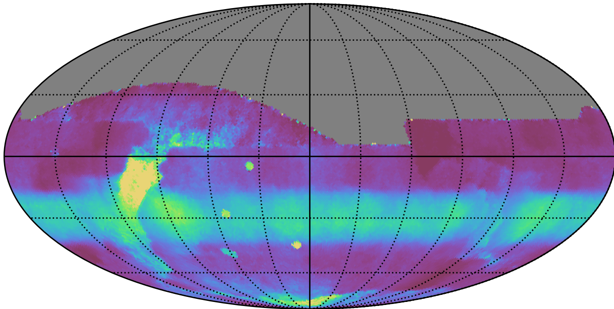
weather_cloudso8v3.4_10yrs All sky all bands: Median normairmass
