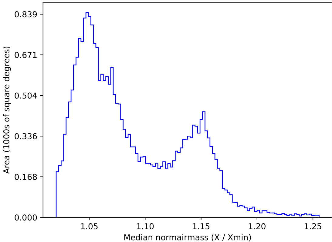
weather_cloudso8v3.4_10yrs All sky all bands: Median normairmass
