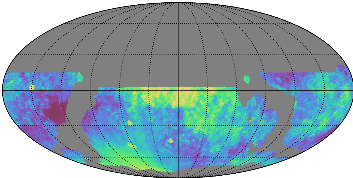
weather_cloudso8v3.4_10yrs WFD z band: Median moonDistance
