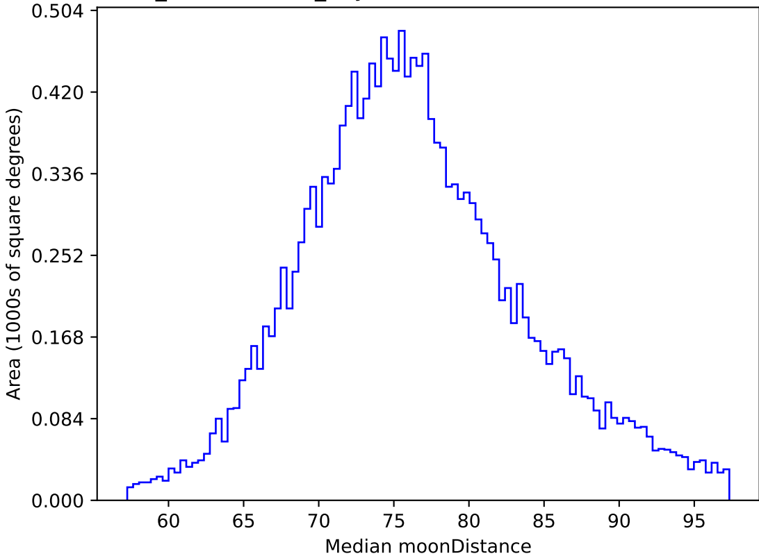
weather_cloudso8v3.4_10yrs WFD z band: Median moonDistance
