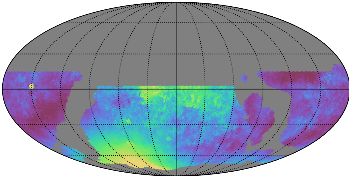
weather_cloudso8v3.4_10yrs WFD y band: Median moonDistance
