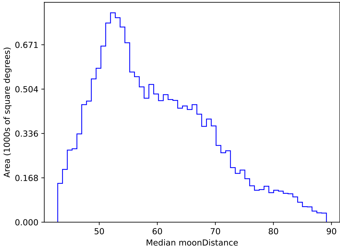
weather_cloudso8v3.4_10yrs WFD y band: Median moonDistance
