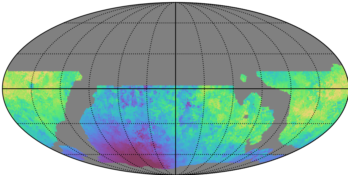
weather_cloudso8v3.4_10yrs WFD u band: Median moonDistance
