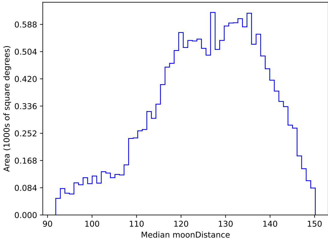
weather_cloudso8v3.4_10yrs WFD u band: Median moonDistance
